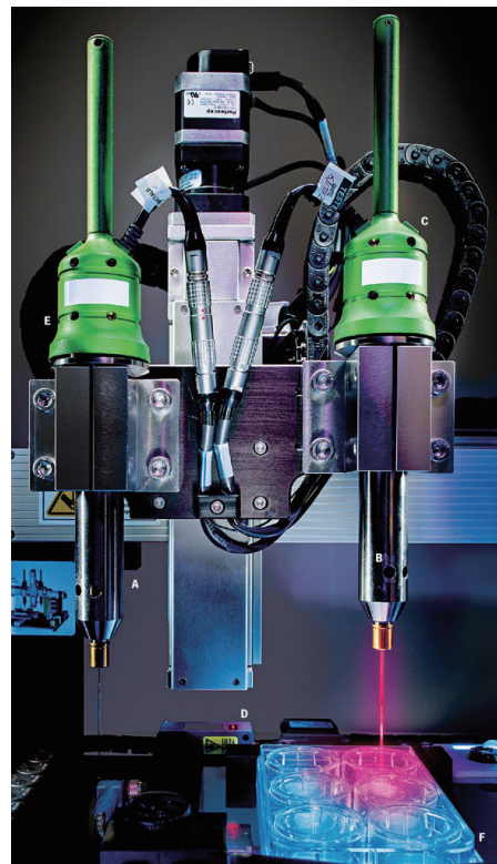
NovoGen MMX bioprinter © Popular Science
