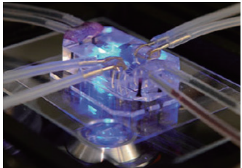
An organ-on-a-chip © Wyss Institute
